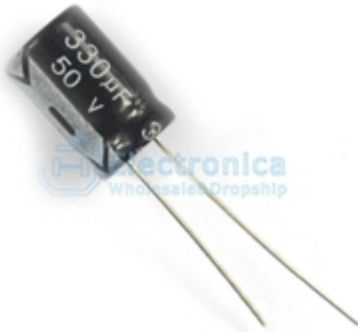
Electrolytic Capacitor 50V/330UF 10*17MM
